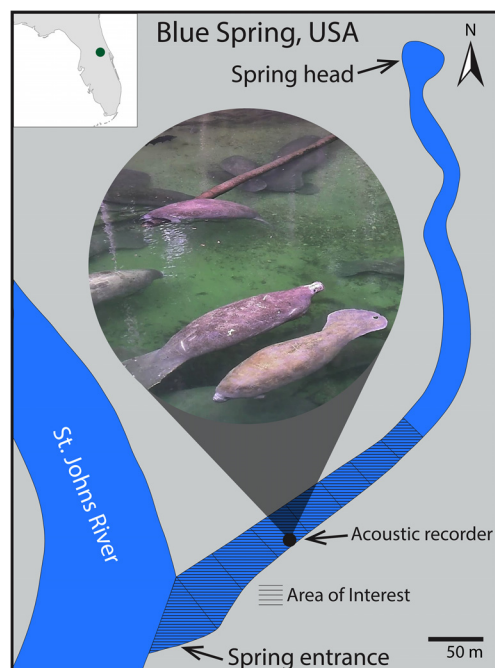
Fig. 1. A diagram of the study area. The acoustic recorder (black circle; 28.9438^{\circ}\text{N} , -81.3405^{\circ}\text{W} ) was deployed in the Blue Spring run in Florida, USA (inset in the top left corner shows Florida, USA, with a green circle indicating the location of Blue Spring). The narrow run leads to a natural warm-water spring at the North end. The clear water (inset picture) allows for visual counts of the manatees using the spring run. The hatched area represents the combined zones (zones are demarcated by black lines) from which visual manatee counts were grouped to estimate the number of manatees within acoustic range of the recorder (Area of Interest). The area of interest is 286 m in length. The contours of the spring run and St. Johns River were traced from Google earth imagery (Google Earth, 2021).
