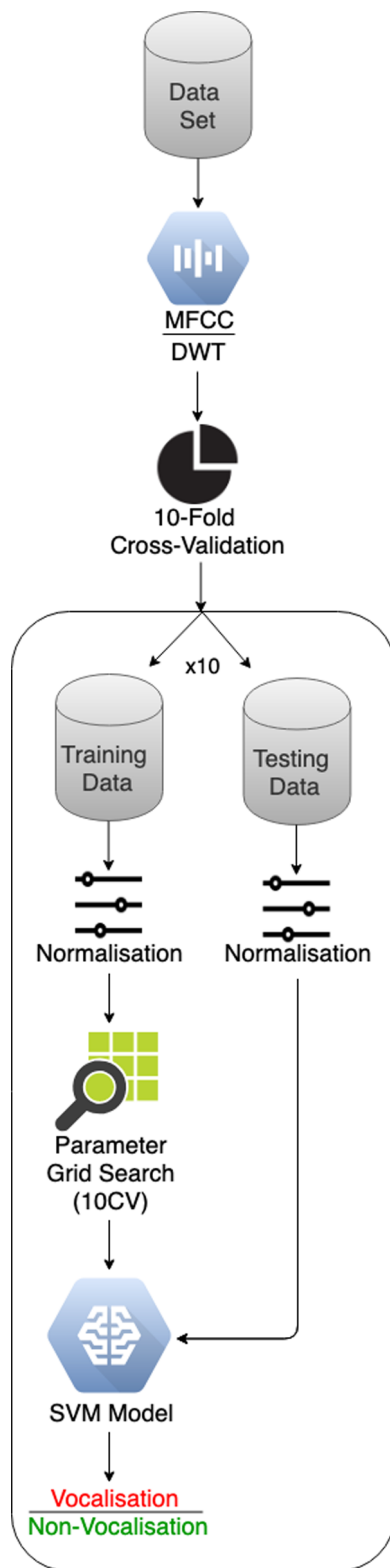
Fig. 8. Overview of algorithm training and testing procedure.
