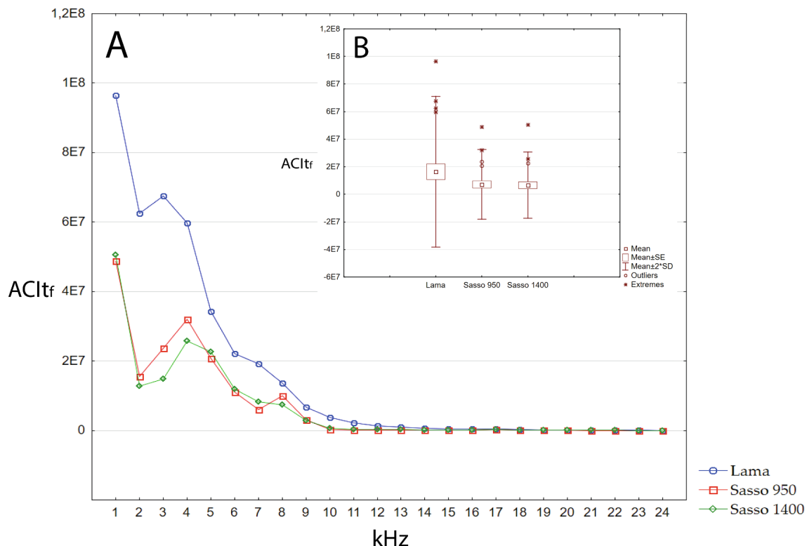
Fig. 3. (A) Distribution of ACItf when aggregated according to 1-kHz frequency classes and (B) descriptive statistics for Lama, Sasso 950 and Sasso 1400.
