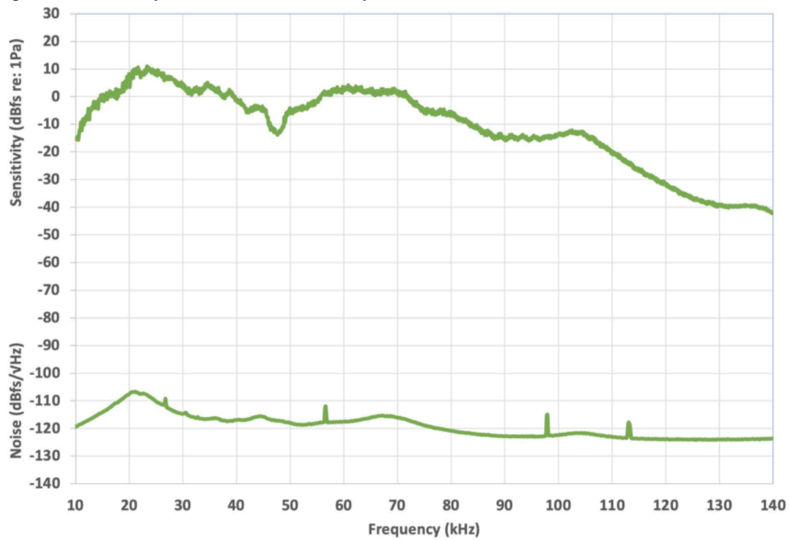
Figure 18. Sensitivity and Noise of the SMART System with SMART MIC-1
