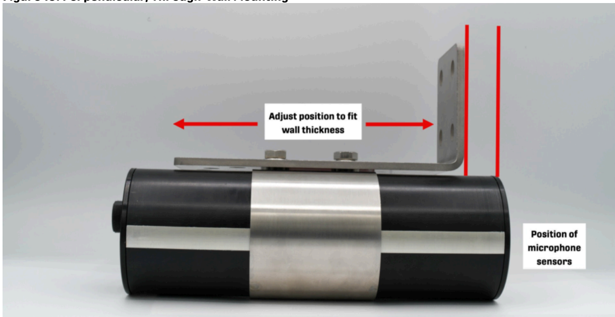
Figure 10. Perpendicular, Through-Wall Mounting
