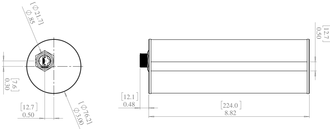
Figure 17. SMART MIC-1 Dimensional Drawings.
