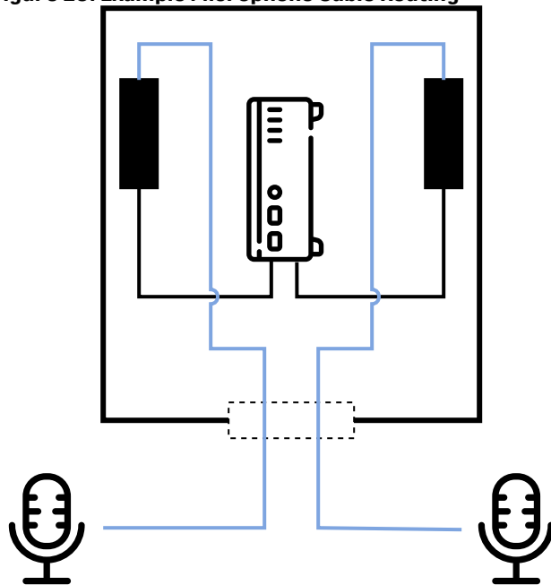
Figure 20. Example Microphone Cable Routing
