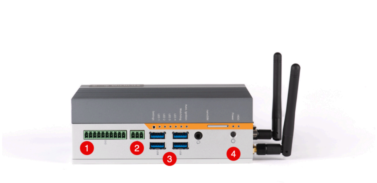
Figure 3. SMART Controller Connectivity: Digital I/O, USB, and Power Button
