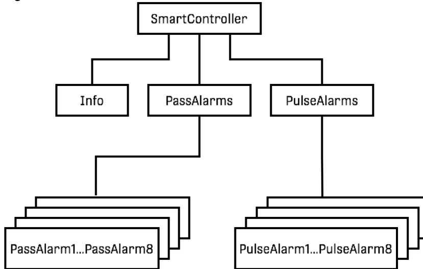
Figure 14. OPC UA Information Model Overview
