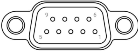
Figure 15. Serial Port Pin Arrangement
