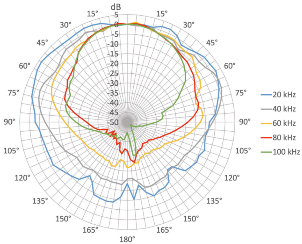
Figure 19. Directionality of the SMART System with SMART MIC-1
