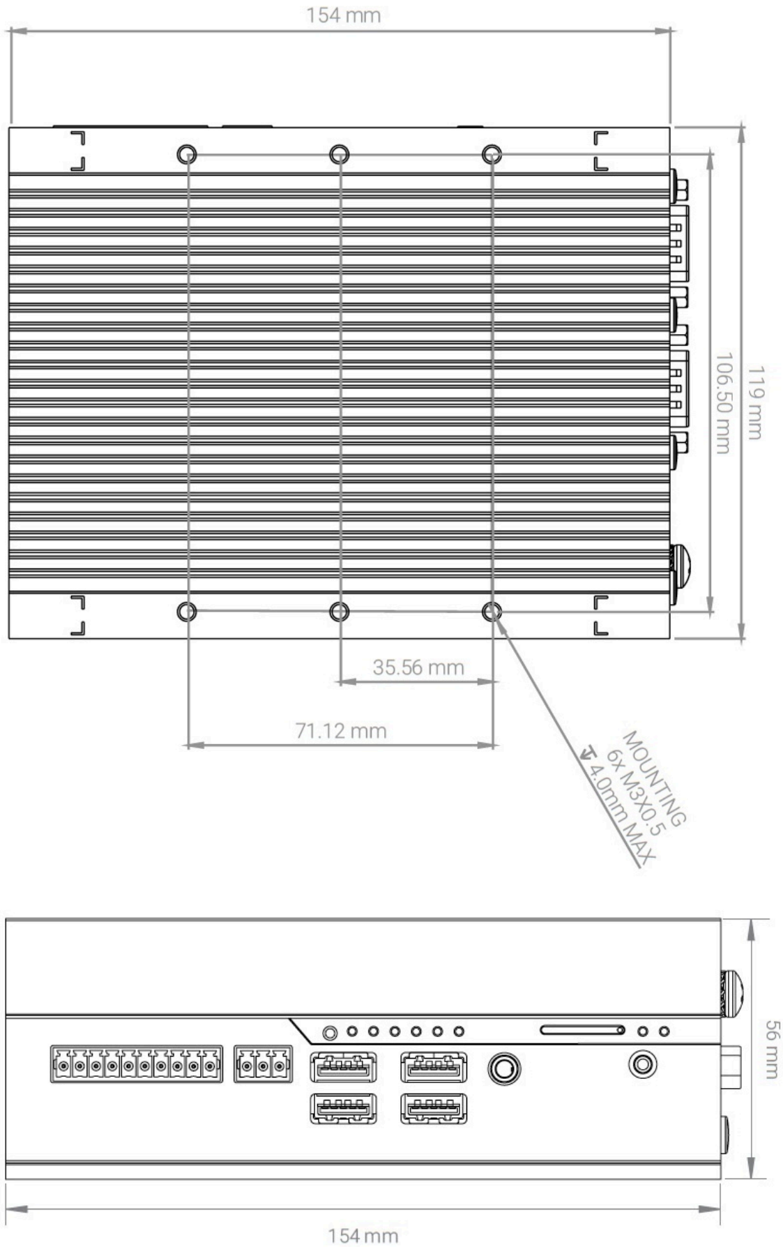
Figure 16. SMART Controller Dimensional Drawings, with Mounting Points
