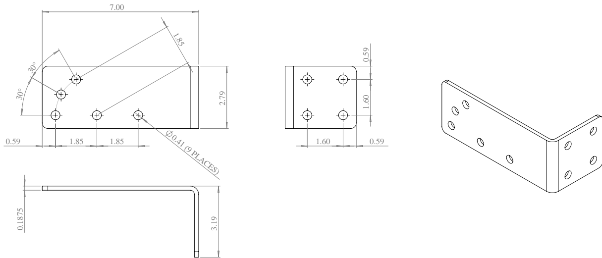
Figure 9. SMART MIC-1 Mounting Bracket Dimensional Drawings
